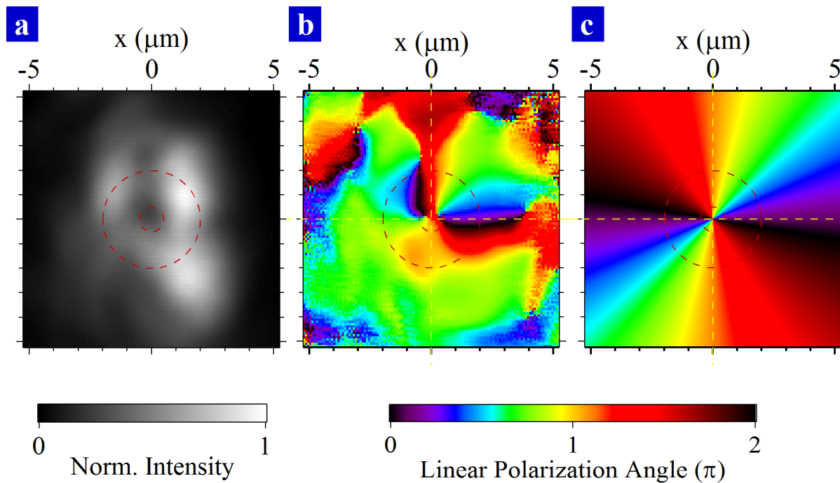
Figure 3 Imaging of a Spin Vortex. (a) Time-integrated real-space condensate density. The core of the spin vortex can be identified at the center of the smaller red circle. (b) Linear polarization angle map, indicating the direction of the linear polarization, when circumventing the spin vortex core in the Stokes parameters space (by definition, a rotation of 2\pi in real space corresponds here to the doubled 4\pi rotation we observe). A good agreement is found between the experimental result and the theoretical simulation, which is shown in (c). The red dashed circles and the yellow lines serve as a guide for the eye to identify the vortex position.
