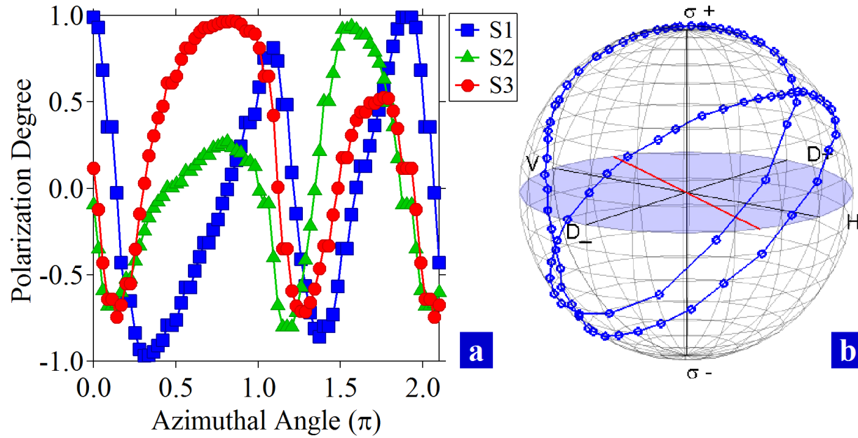
Figure 5 Trajectories in the Poincaré sphere. (a) Polarization degree profiles around the vortex core the horizontal-vertical ( S_1 ), diagonal ( S_2 ) and circular ( S_3 ) bases. The unpolarized emission has been removed (see Supplementary Figure S4). (b) Representation in the Poincaré sphere of the double rotation of the Stokes vector of the condensate polarization, when circumventing the spin vortex core.
