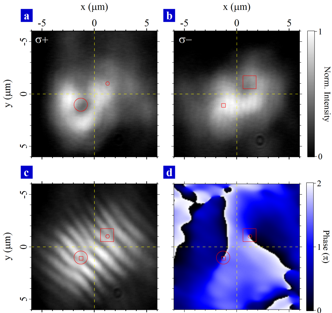
Figure 2 Spin vortex interferometric signature. The real-space density of \sigma+ (a) and the retroreflected \sigma- (b) components of the condensate are overlapped in the polarization mixing interferometer to obtain the interference pattern (c). The corresponding phase structure is shown in (d). The polarization vortex interferometric signature consists in a pair of co-oriented fork-like dislocations, appearing at centrosymmetric positions with respect to the autocorrelation point. The red circle (for \sigma+ ) and square (for \sigma- ) indicate the phase dislocation positions (large marker) and their corresponding centrosymmetric position (small marker). The yellow dashed lines cross at the autocorrelation point, central point of symmetry.
