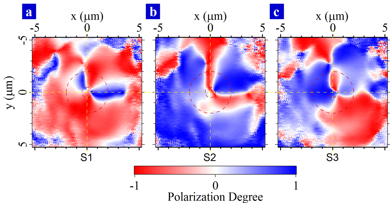
Figure 4 Spin textures. Polarization rate (Stokes parameter) maps along the horizontal-vertical (a), diagonal (b) and circular (c) bases. The unpolarized emission has been removed (see Supplementary Figure S4).
